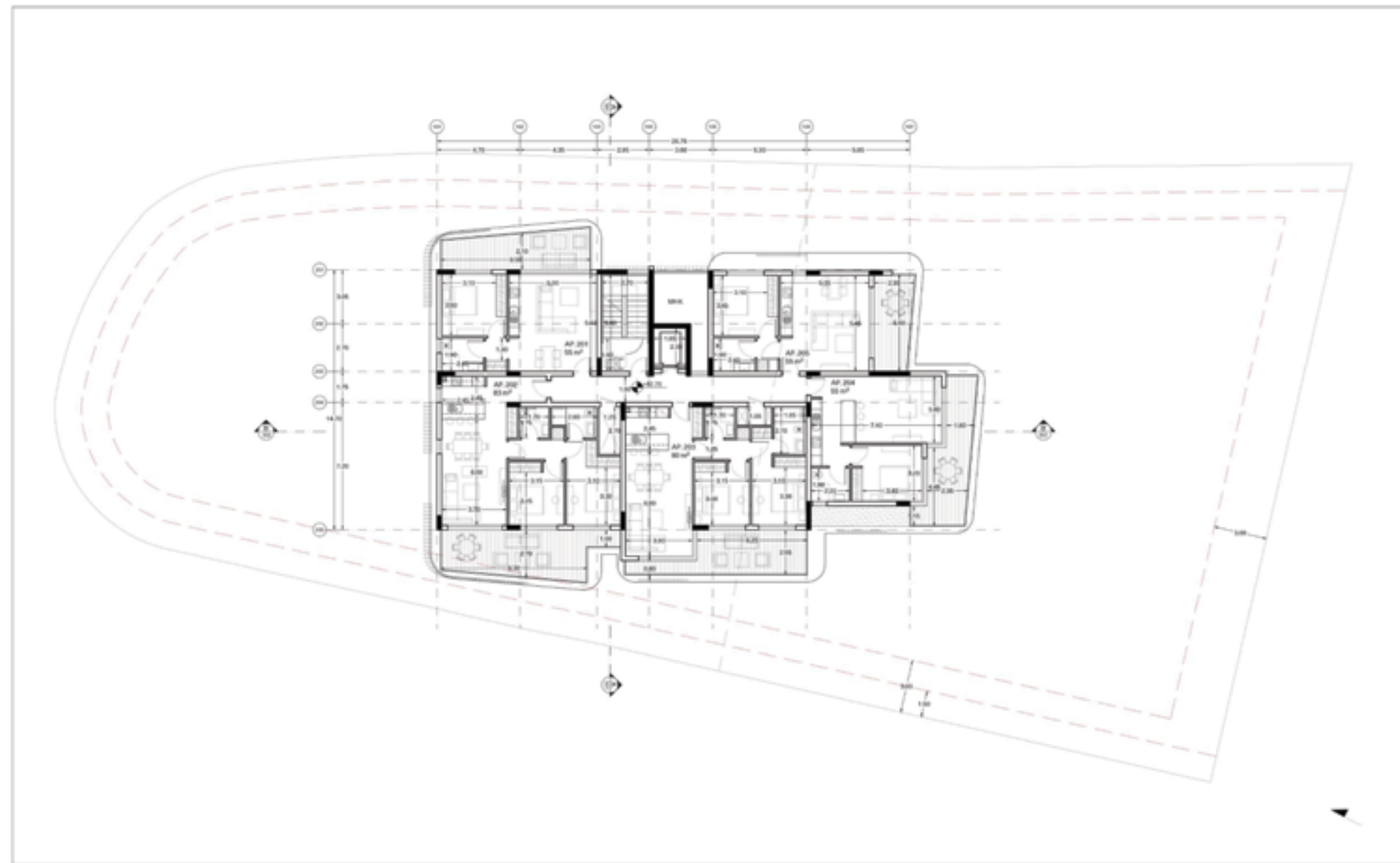
Second Floor: Three 1-Bedroom Apartments | Two 2-Bedroom Apartments
